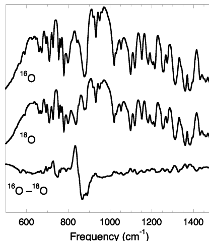
Figure 2. Infrared spectra of KBr pellets of [L^{tBu}Fe]_2O and its ^{18}O isotopomer. Vertical scaling of the subtraction has been increased for clarity.
