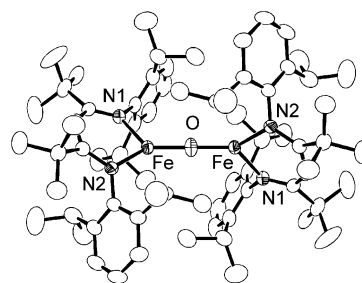
Figure 1. Thermal ellipsoid plot of [L^{tBu}Fe]_2O \cdot OEt_2 (50% probability ellipsoids), viewed along the C_2 axis. Hydrogen atoms and unassociated diethyl ether are omitted for clarity. Relevant distances (Å) and angles (deg): Fe-O 1.7503(4), Fe-N1 2.005(2), Fe-N2 1.966(2), Fe-O-Fe 167.55(14) , N1-Fe-N2 98.22(7) .
